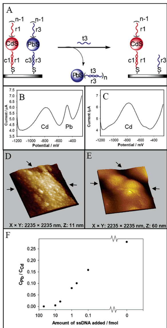
Figure 2. Competition assay for detection of DNA target t3 (50 fmol in 3 mL) (A) and anodic stripping voltammetry analysis of the particles remaining at the surface before (B) and after (C) addition of t3 . AFM images of an area covered with the PbS- r3 nanoparticle complexed to the immobilized c3 sequence (D), and the same area after addition of the competing DNA target t3 (E). That the imaging was carried out on the same area is evident from the depressions observed in the areas indicated with dotted arrow marks. Ratio between the areas (charge) of the Pb and Cd peaks obtained by stripping voltammograms performed after addition of 50 to 0.1 fmol of t3 and in the absence of t3 (F).
